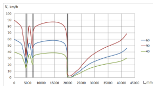
Figure 8 – Figure velocity of the air around the main road trains with low cab with improved fairing behind
