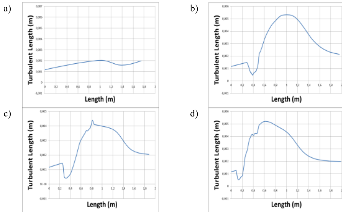
Figure 4 – The schedules of turbulence scale changes l_m (m) relatively to the tube axis L (m) (curves l_m(L) ):
